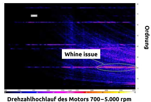
Analyse Gear whine
